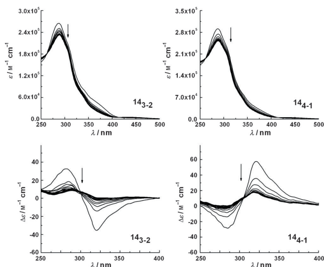
Figure 2. UV/Vis absorption (top) and CD (bottom) spectra indicate photochemical E \rightarrow Z isomerization of oligomers 14 3,2 and 14 4,1 during irradiation ( \lambda_{\text{irr}} = 358 nm) in \text{CH}_3\text{CN} at 25 °C.
